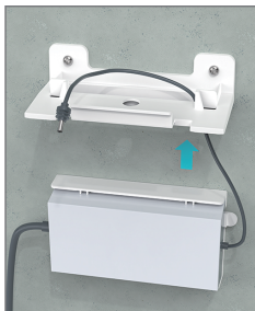
2. Power cord runs underneath through the bracket
