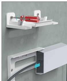
1. Bracket is fixed to the wall and the power supply is pushed into the slot
